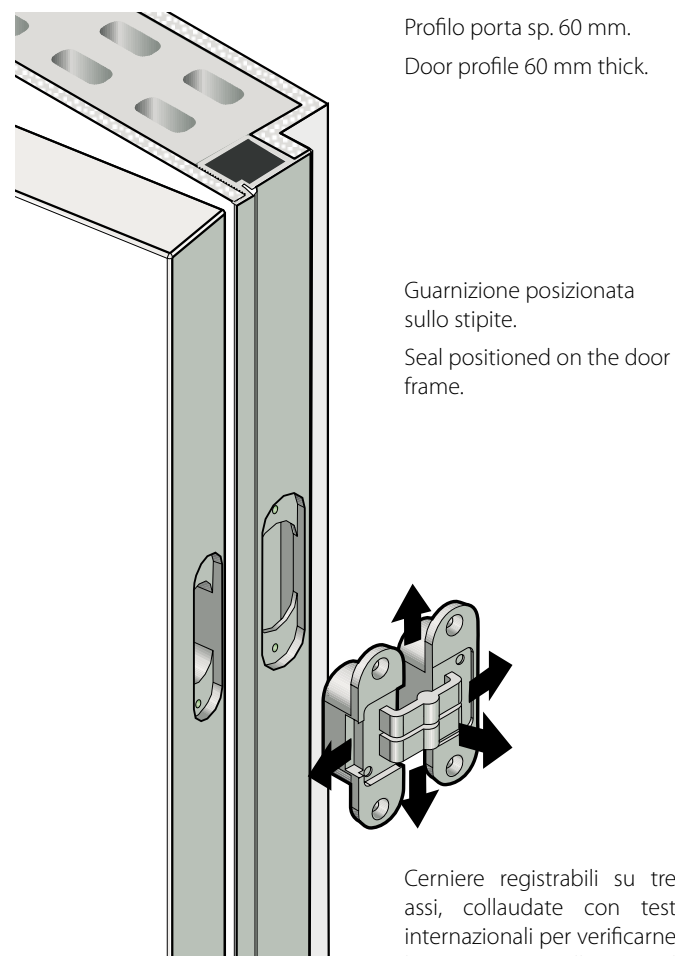
Adjustable hinges on three axes, tested in international tests to ensure resistance to wear over time.
