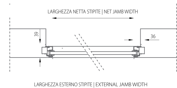
SETTO FISSO CON WALL U A TERRA FIXED PARTITION WITH WALL U TO GROUND
